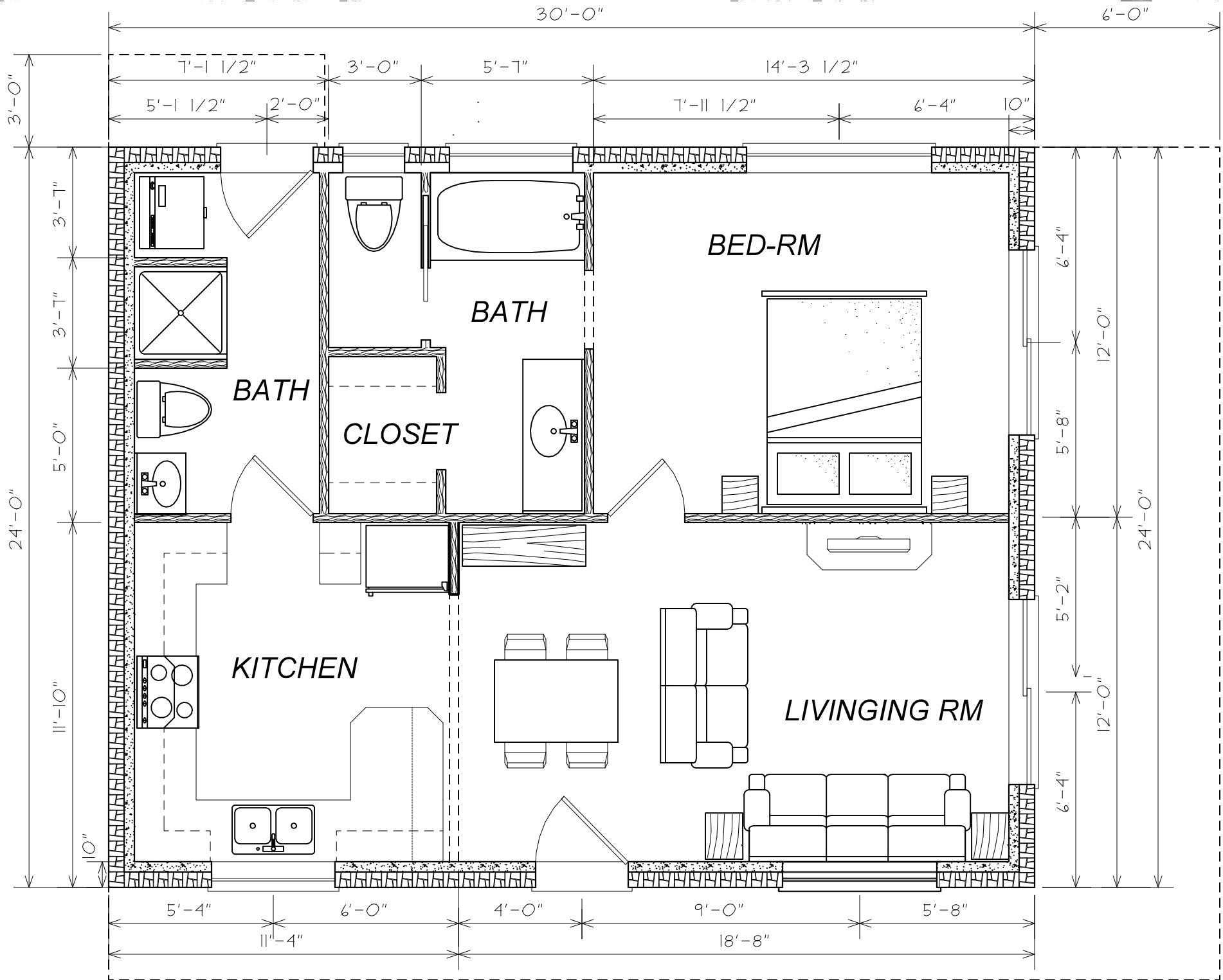
LAKE HOUSE FLOOR PLAN 1/4"=1'
