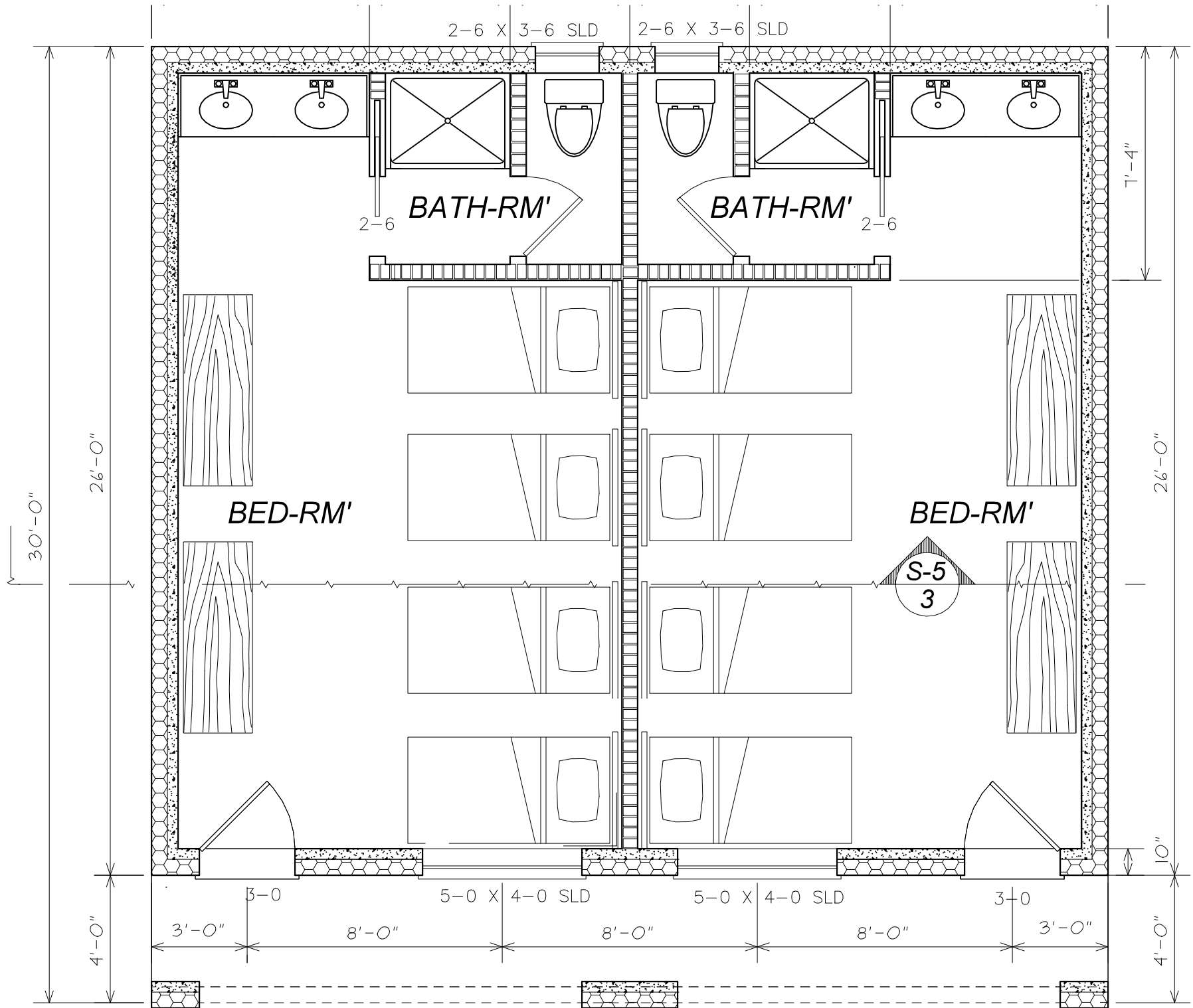
LODGE FLOOR PLAN 1/4"=1'
